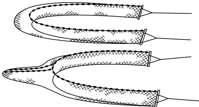
FIGURE 1. — Beach seine diagrams (FAO technical paper). The lower net has a “bag” in the “bunt” (middle) section in order to hold more fish and to prevent fish from escaping. Bunt mesh size is usually smaller than for “wing” sections. Typically “tow lines” are attached to each end to allow pulling the net in from a distance.
