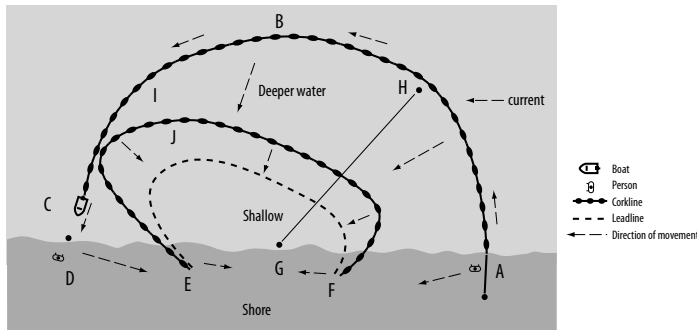
FIGURE 11. — Simple arc set for a beach seine using a motorboat. The seine is initially set from A to B to C. Note that a perfect semicircle is rarely attained (see radii GA, GH, GB, GI and GD in this example) so that area and volume calculations will be approximate. One possible position of the net is shown after half-retrieval (FJE), affected by a current coming from the right and the persons at A and D moving towards each other (note that the lead line is in advance of the cork line). (Illustration: Andrew Fuller from design by Peter Hahn.)
