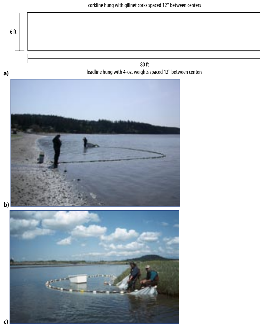
FIGURE 13. — Small net beach seine methodology. (A) Design of net (not to scale); (B) setting the net on a shallow beach; (C) beginning to haul (pursing) the net. (Photos: A—Eric Beamer, Skagit System Cooperative, 2003; B—Karen E. Wolf; C—Richard A. Henderson).
