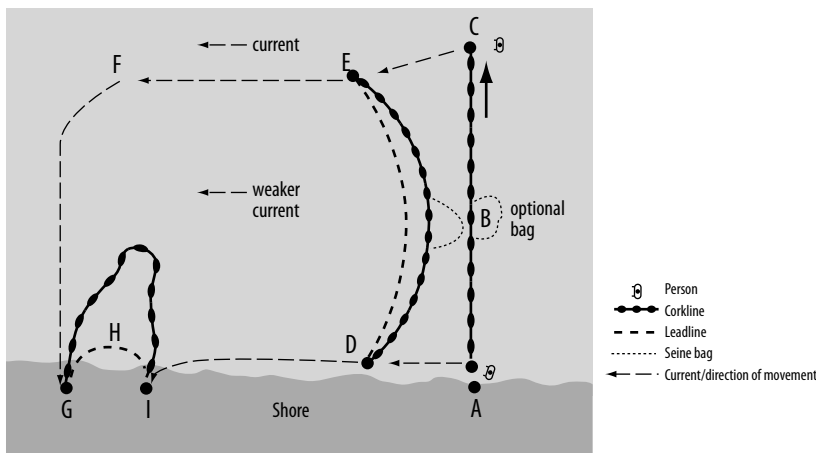
FIGURE 6. — Perpendicular set deployment and retrieval of a beach seine (not to scale). (Note: the distance A–I may be very long—perhaps several hundred meters.) (Illustration: Andrew Fuller from design by Peter Hahn.)
