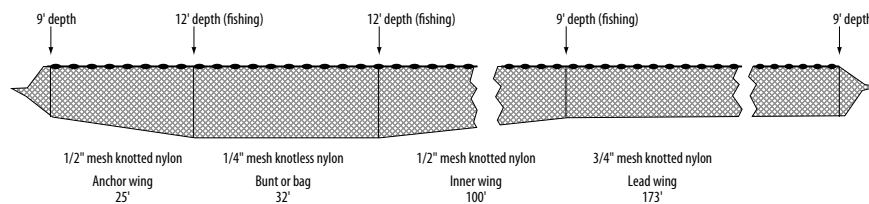
FIGURE 2. — Example of beach seine dimensions with unequal tapered wings (from Sims and Johnsen 1974) used in the Columbia River estuary, Washington. (Illustration: Andrew Fuller, from Sims and Johnsen.)
