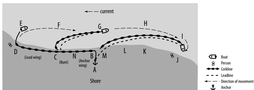
FIGURE 17. — Beach-lay elliptical arc set deployment and retrieval of a beach seine. (Illustration: Andrew Fuller from design by Peter Hahn.)
