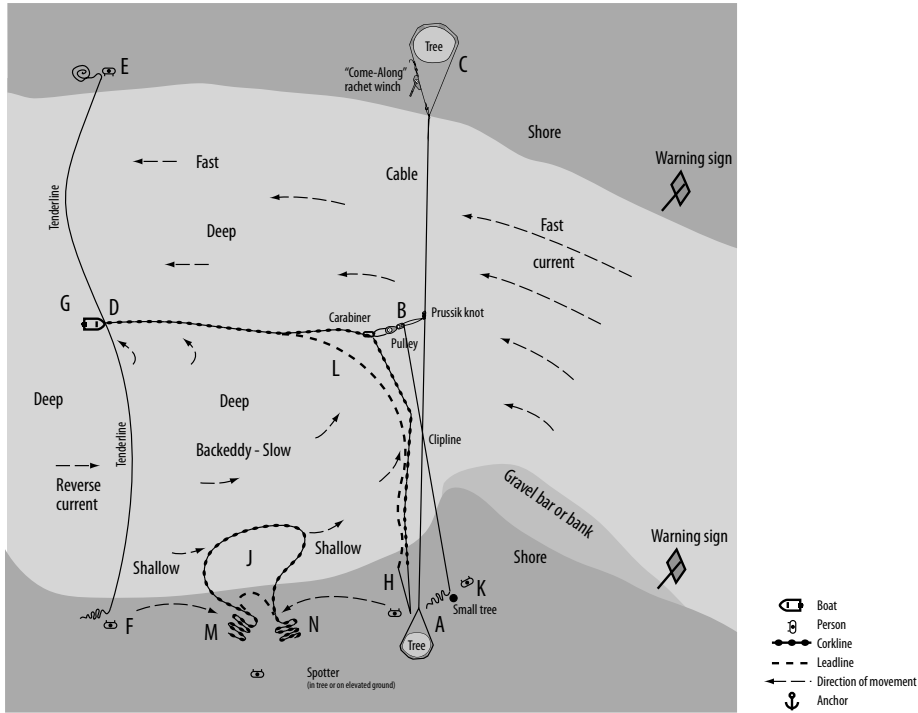
FIGURE 18. — Cable-L trap set with a beach seine to capture adult chinook salmon in the Shuswap River in British Columbia. (Illustration: Andrew Fuller from Richard E. Bailey, Canadian Department of Fisheries and Oceans.)
