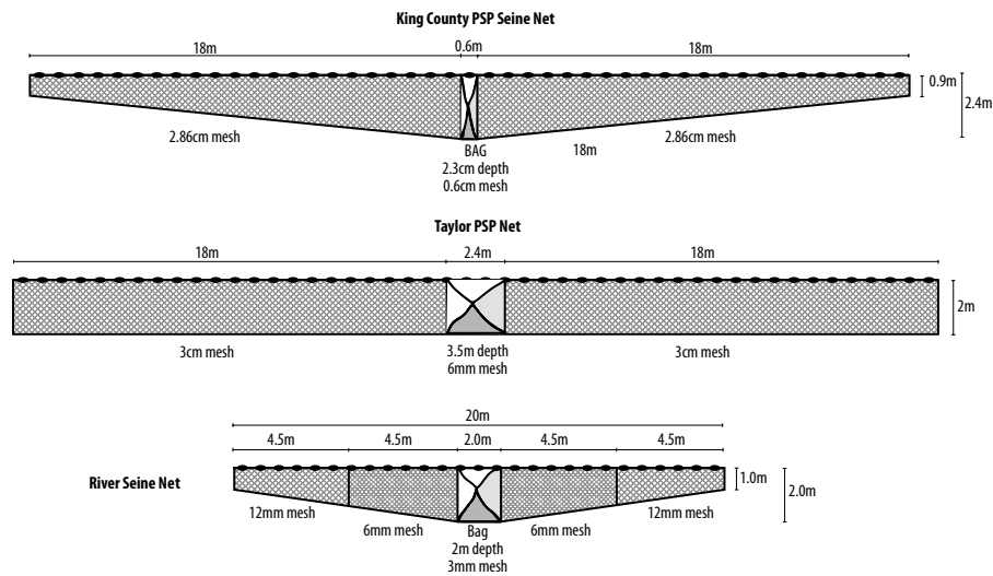
FIGURE 3. — Example of three beach seines used in Puget Sound, Washington. (Illustration: Andrew Fuller from Nelson et al. 2004, King County Department of Natural Resources.)
