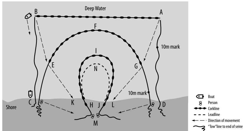
FIGURE 5. — Parallel set deployment and retrieval of a beach seine as used in Puget Sound sampling protocols (not to scale). (Illustration: Andrew Fuller from design by Peter Hahn.)
