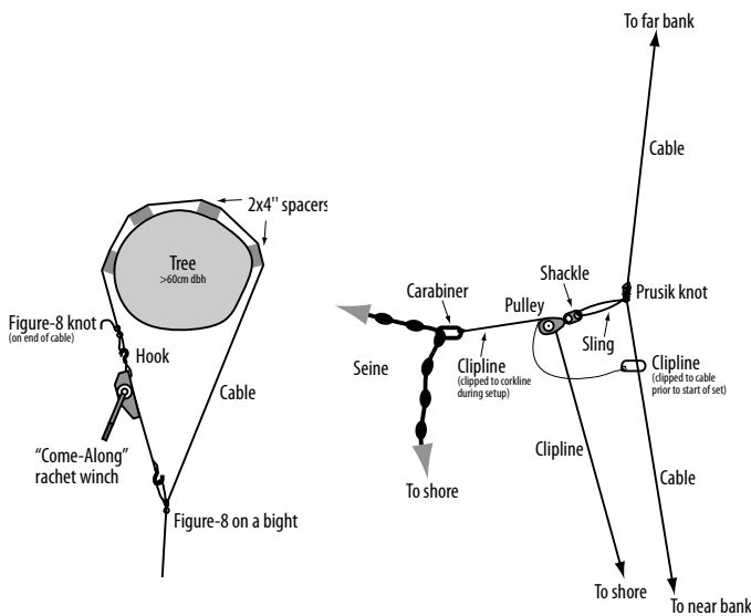
FIGURE 19. — Cable-L trap set details showing (1) how the cable is fixed to sturdy trees on each bank, and (2) how the beach seine is temporarily attached to the middle of the cable, allowing half the seine to stretch downstream. For “Figure-8 on a bight,” see Cox and Fulsaa (2003). (Illustration: Andrew Fuller from design by Peter Hahn.)
